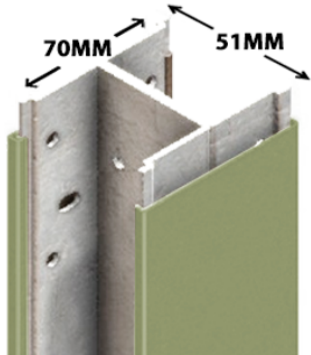
STEEL POST WITH COVER STRIP
